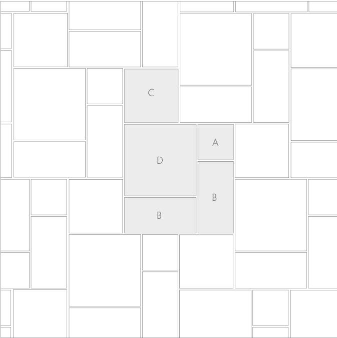
Bourdeaux Pattern one complete pattern equals 11 1/4 sq/ft A (1 pc) 12" X 12" B (2 pcs) 12" X 24" C (1 pc) 18" X 18" D (1 pc) 24" X 24" ‡ bourdeaux pattern available in jerusalem bone
