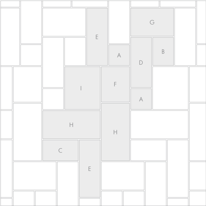
Tourne Pattern one complete pattern equals 28 sq/ft A (2 pcs) 12" X 12" B (1 pcs) 12" X 16" C (1 pcs) 12" X 20" D (1 pcs) 12" X 28" E (2 pcs) 12" X 32" F (1 pcs) 16" X 20" G (1 pcs) 16" X 24" H (2 pcs) 16" X 32" I (1 pcs) 20" X 24"
